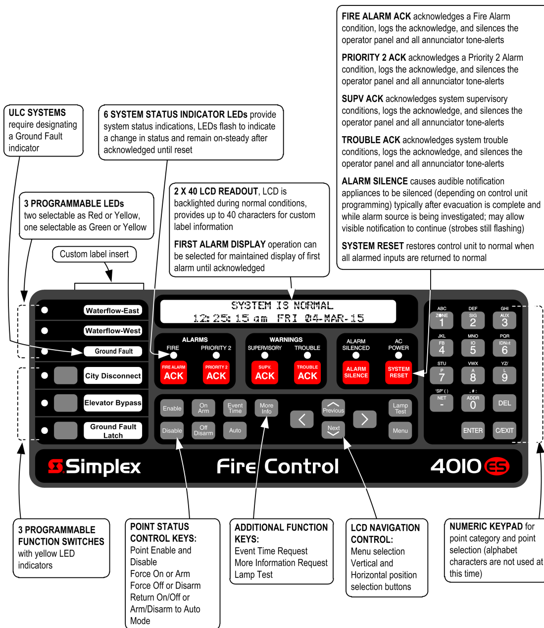
Figure 6: Operator Interface Features
