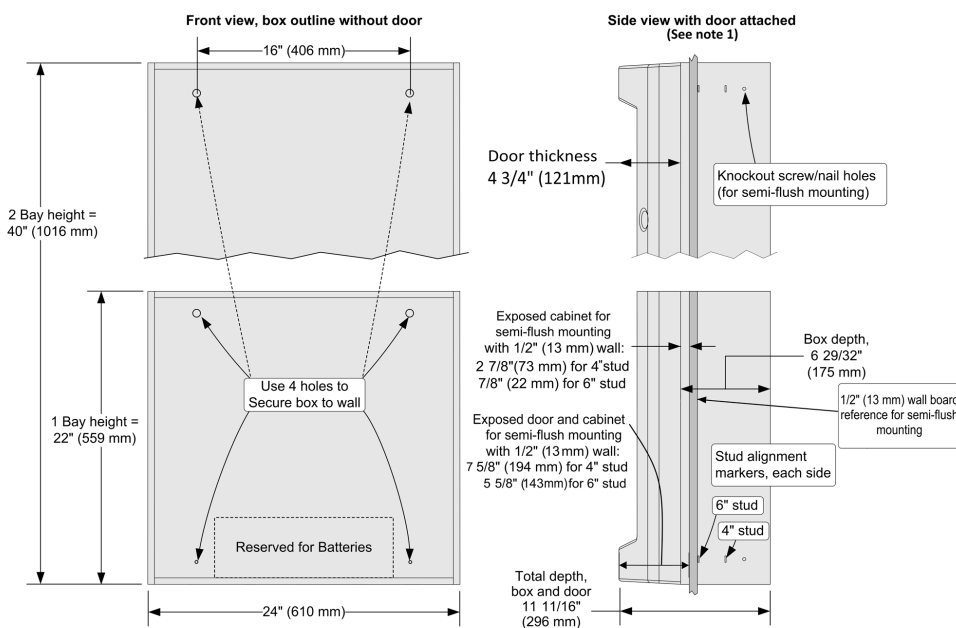
Figure 8: Cabinet dimension reference
