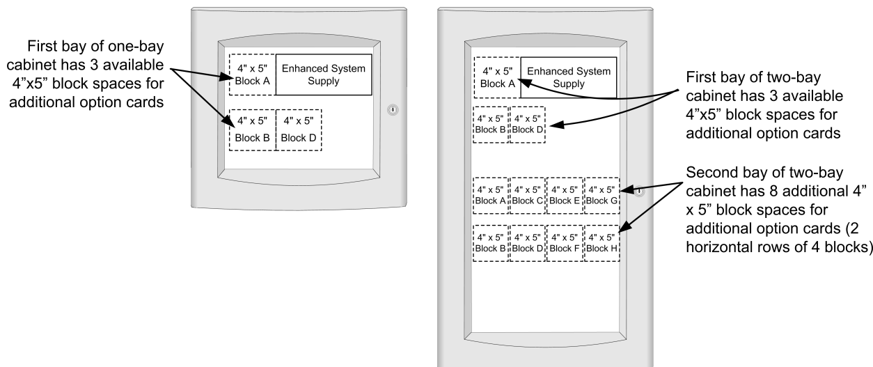
Figure 7: Cabinet One and Two Bay Loading Reference
