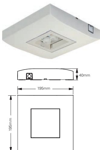
GuideLed SL 13852 CGLine+
